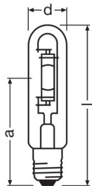
HQI-T 250 W/D PRO
